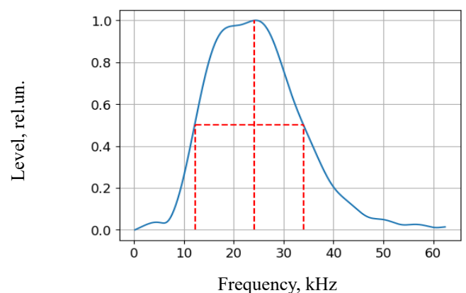
Amplitude-frequency response
