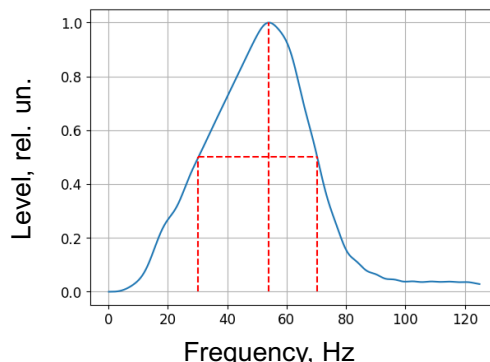
Amplitude-frequency response
